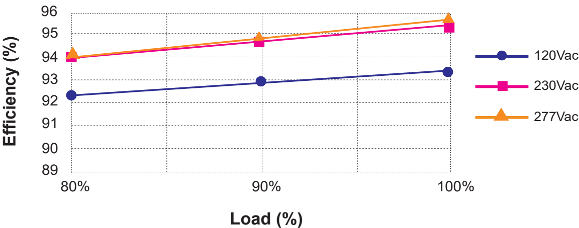
Efficiency Vs Load I_o=16.67A
