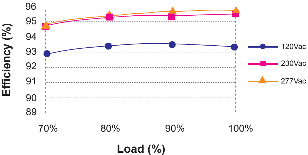
Efficiency Vs Load I_o=14.29A
