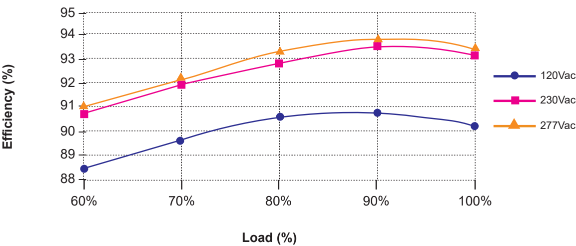
Efficiency Vs Load: I_o = 6.67A
