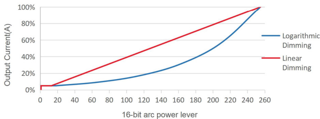
DMX Dimming Curve
