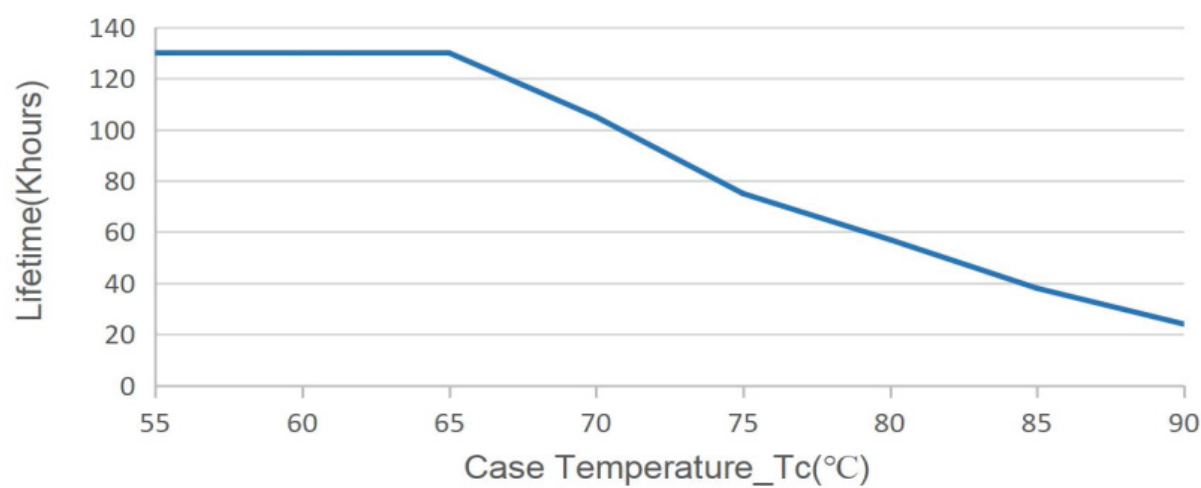
Lifetimes vs Case Temperature
