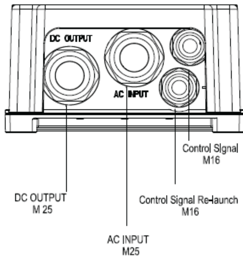
Wire Ports
