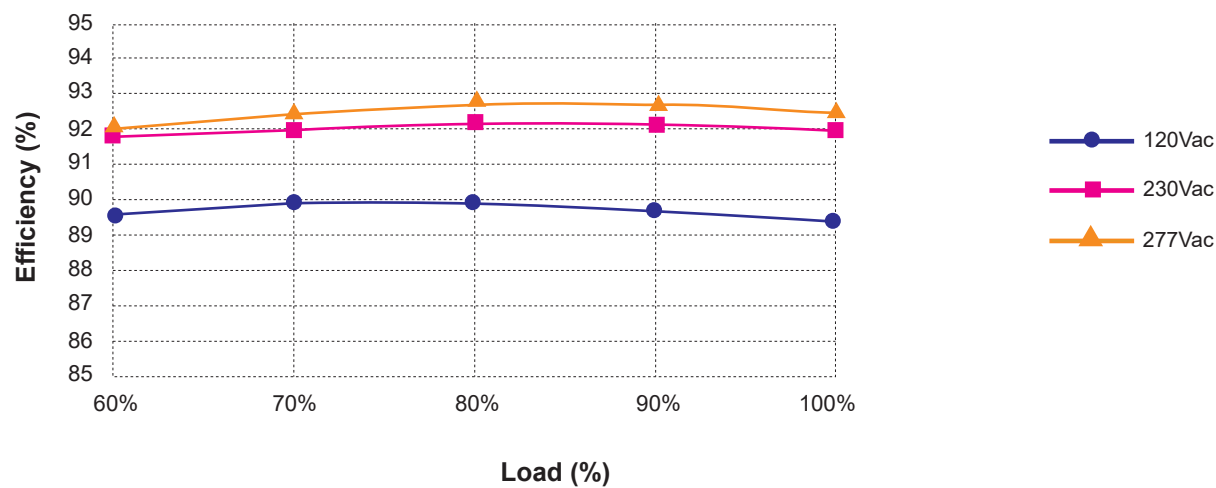
Efficiency Vs Load: I_o = 7.50A
