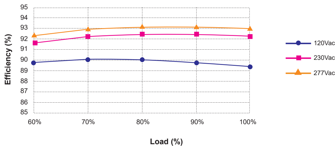
Efficiency Vs Load: I_o = 5.20A
