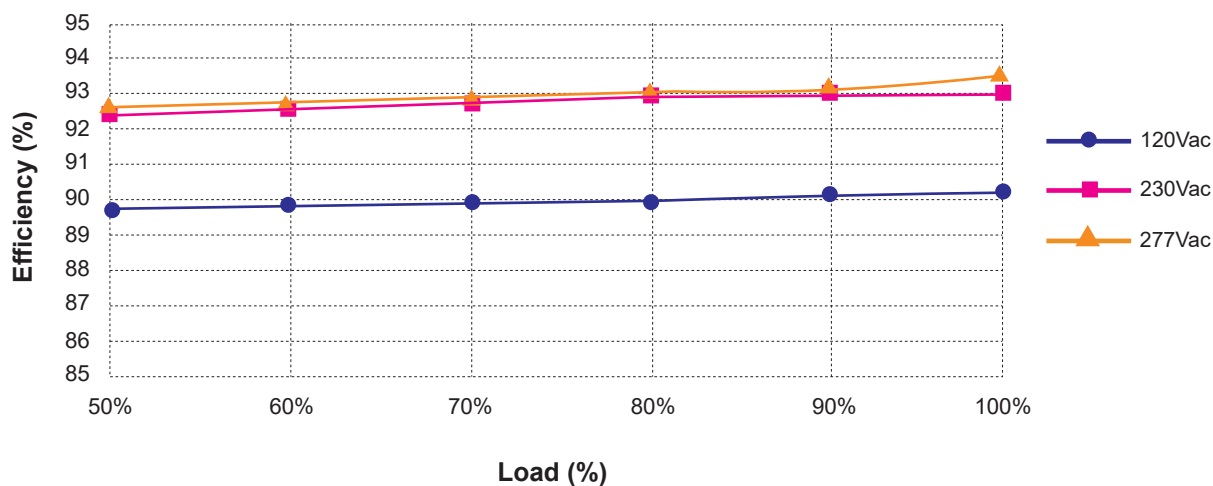
Efficiency Vs Load: I_o = 5.71A
