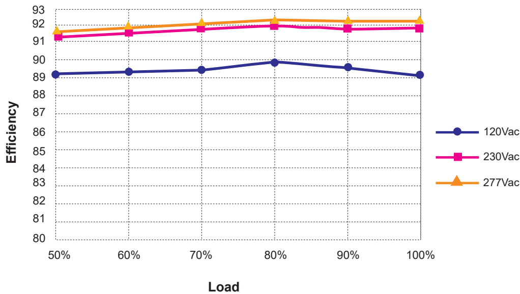
Efficiency Vs Load: I_o = 1.69A
