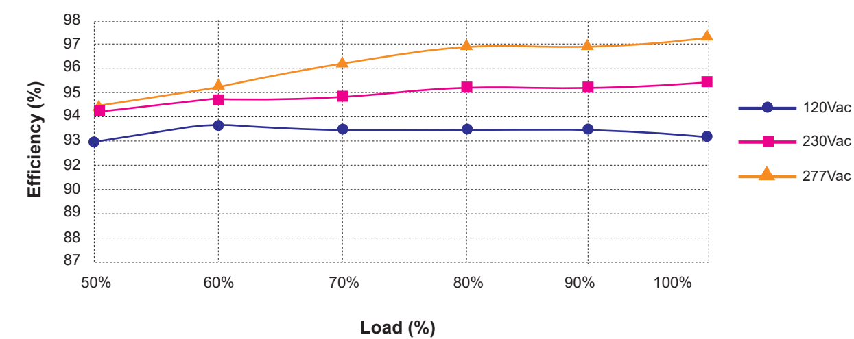
Efficiency Vs Load Io=12.15A
