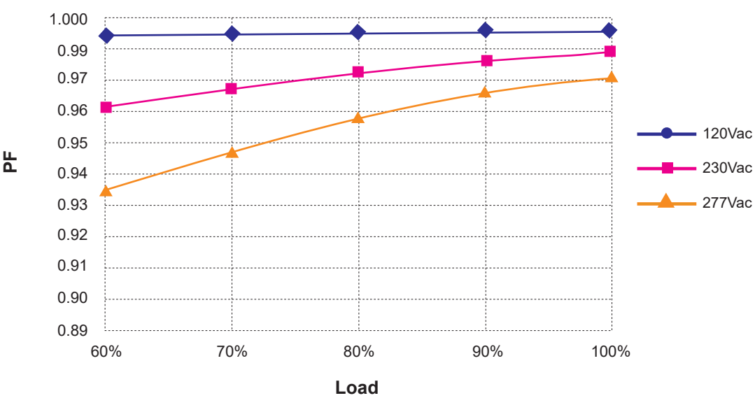
Power Factor Vs Load
