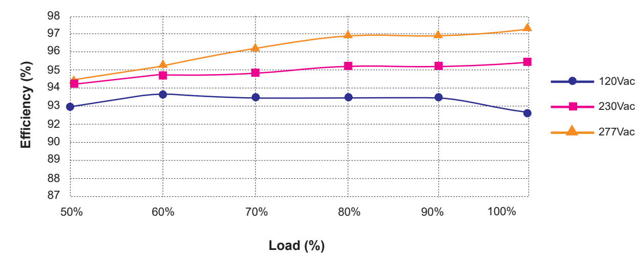
Efficiency Vs Load Io=15.0A
