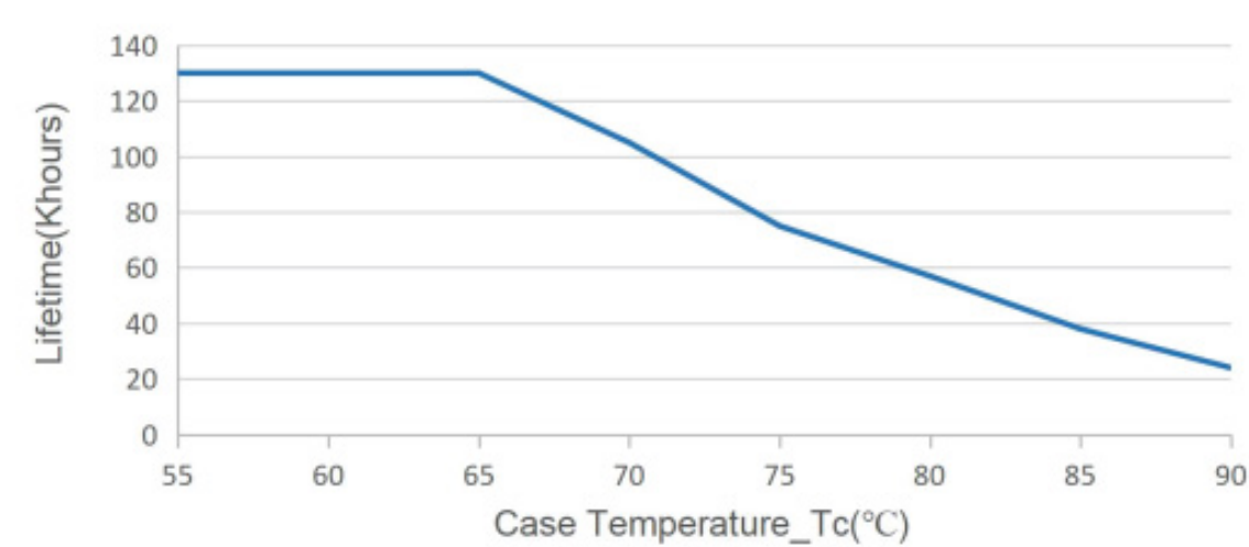
Lifetimes vs Case Temperature
