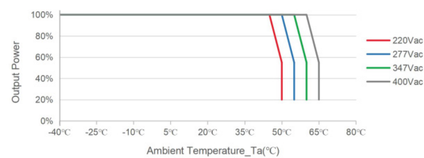
Output Power vs Load Ambient Temperature
