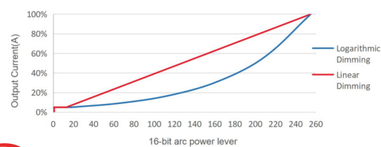
DMX Dimming Curve
